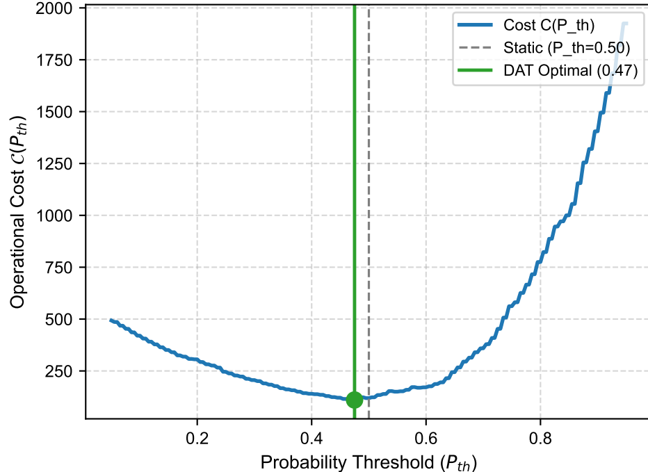
(b) ns-3 Simulated Network Cost Minimisation
