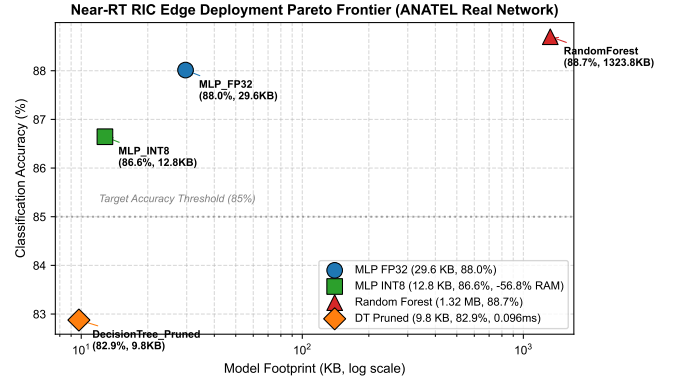
Fig. 5. Near-RT RIC Edge Pareto Frontier displaying trade-offs between model memory footprint (KB), classification accuracy (%), and latency.
