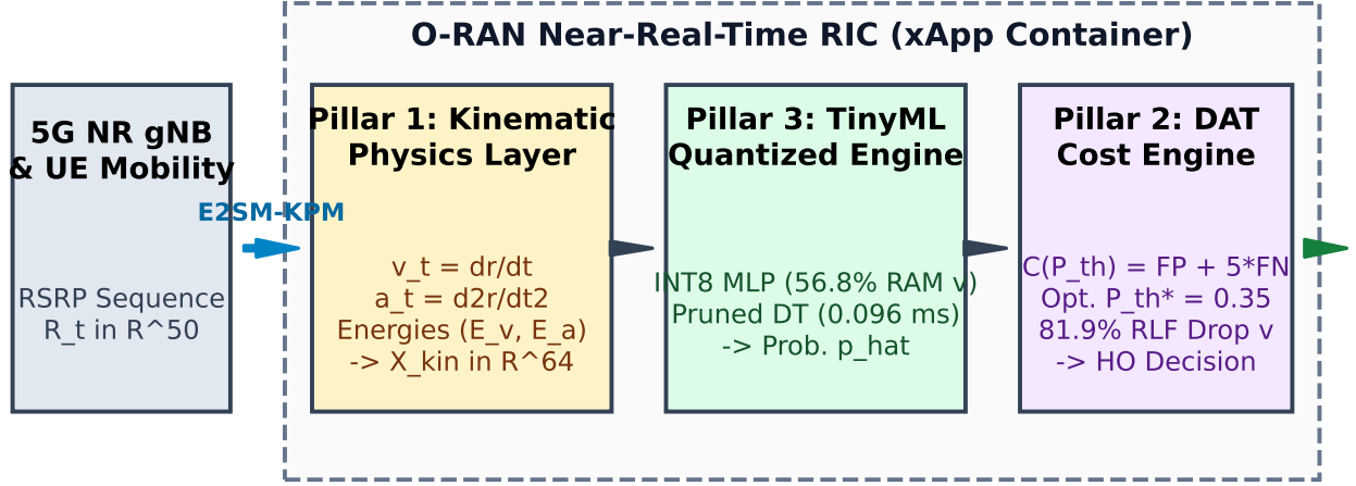
Fig. 1. End-to-End System Architecture of the 3-Pillar Handover xApp operating on the O-RAN Near-Real-Time RIC. Measurements from 5G gNBs ( R_t ) are processed by Pillar 1 (Kinematic Layer), classified by Pillar 3 (TinyML INT8 Engine), and converted into optimal handover trigger commands by Pillar 2 (DAT Cost Engine).
