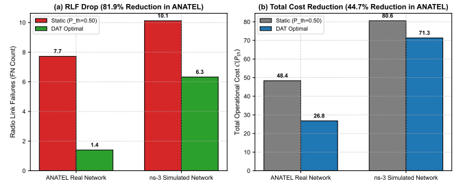
Fig. 4. Comparison of (a) Radio Link Failures (FN) and (b) Total Operational Cost \mathcal{C}(P_{th}) between Static baseline ( P_{th} = 0.50 ) and DAT Optimal.
