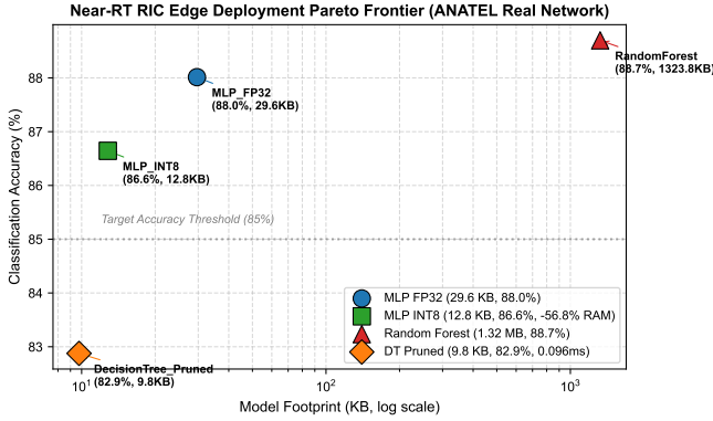
Fig. 5. Near-RT RIC Edge Pareto Frontier displaying trade-offs between model memory footprint (KB), classification accuracy (%), and latency.
