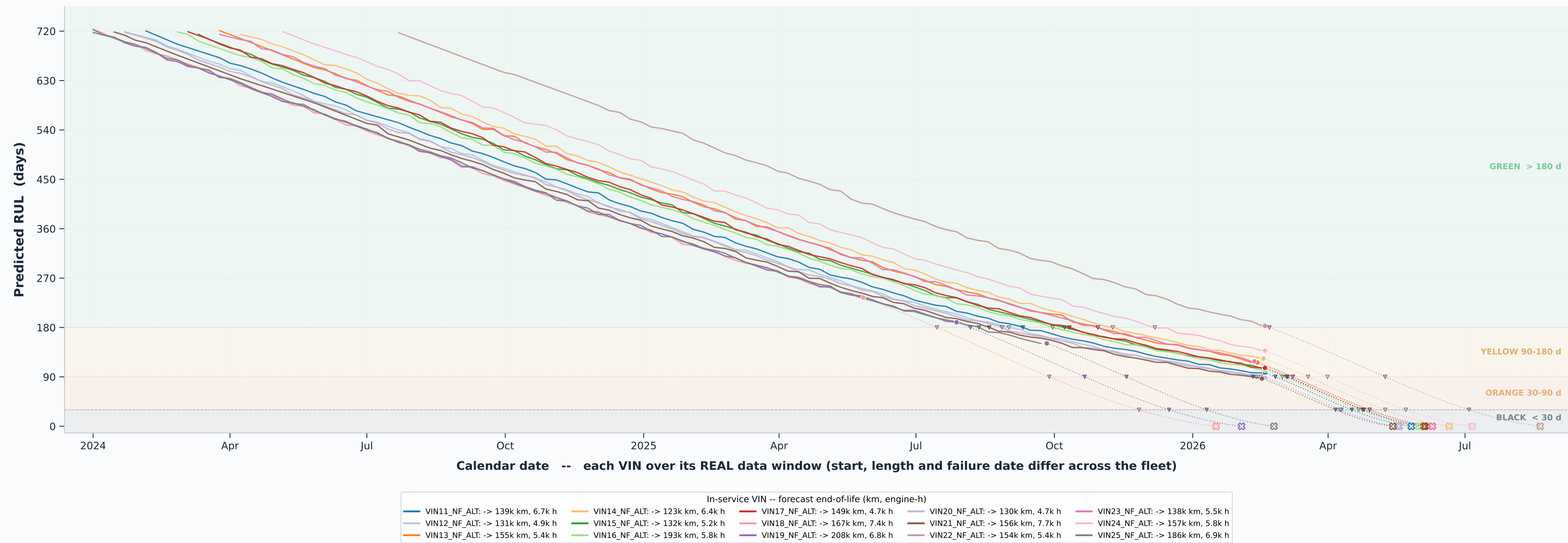
IN-SERVICE alternators (n=15) -- observed (solid) + forecast (dotted)
