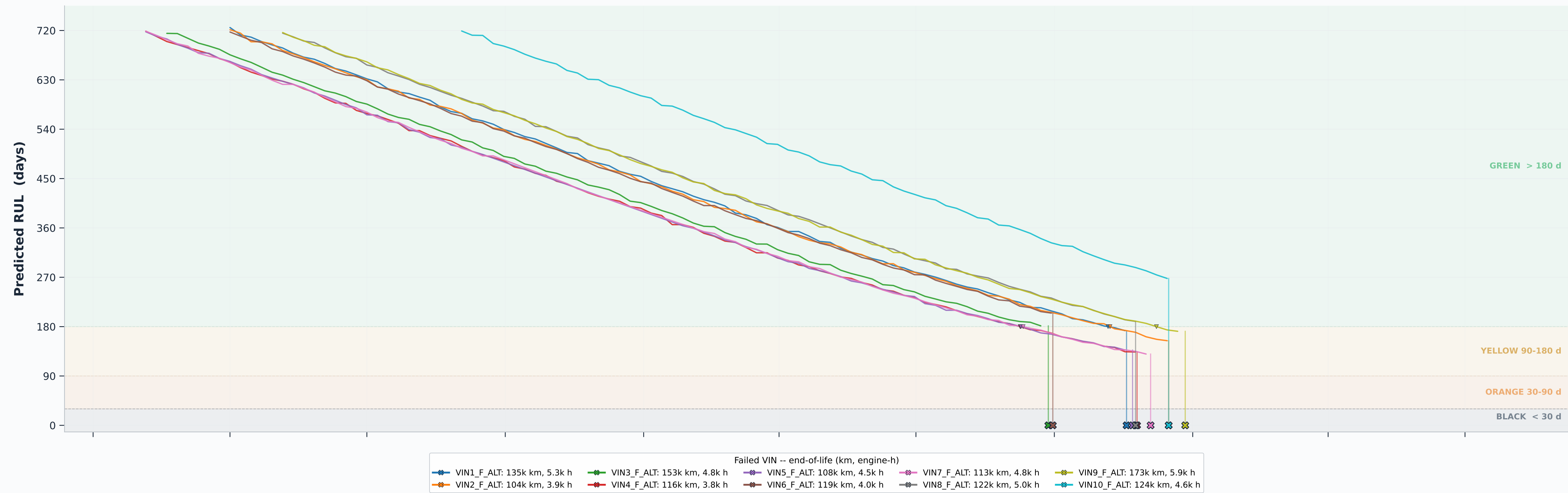
FAILED alternators (n=10) -- real data window, X at realised failure
