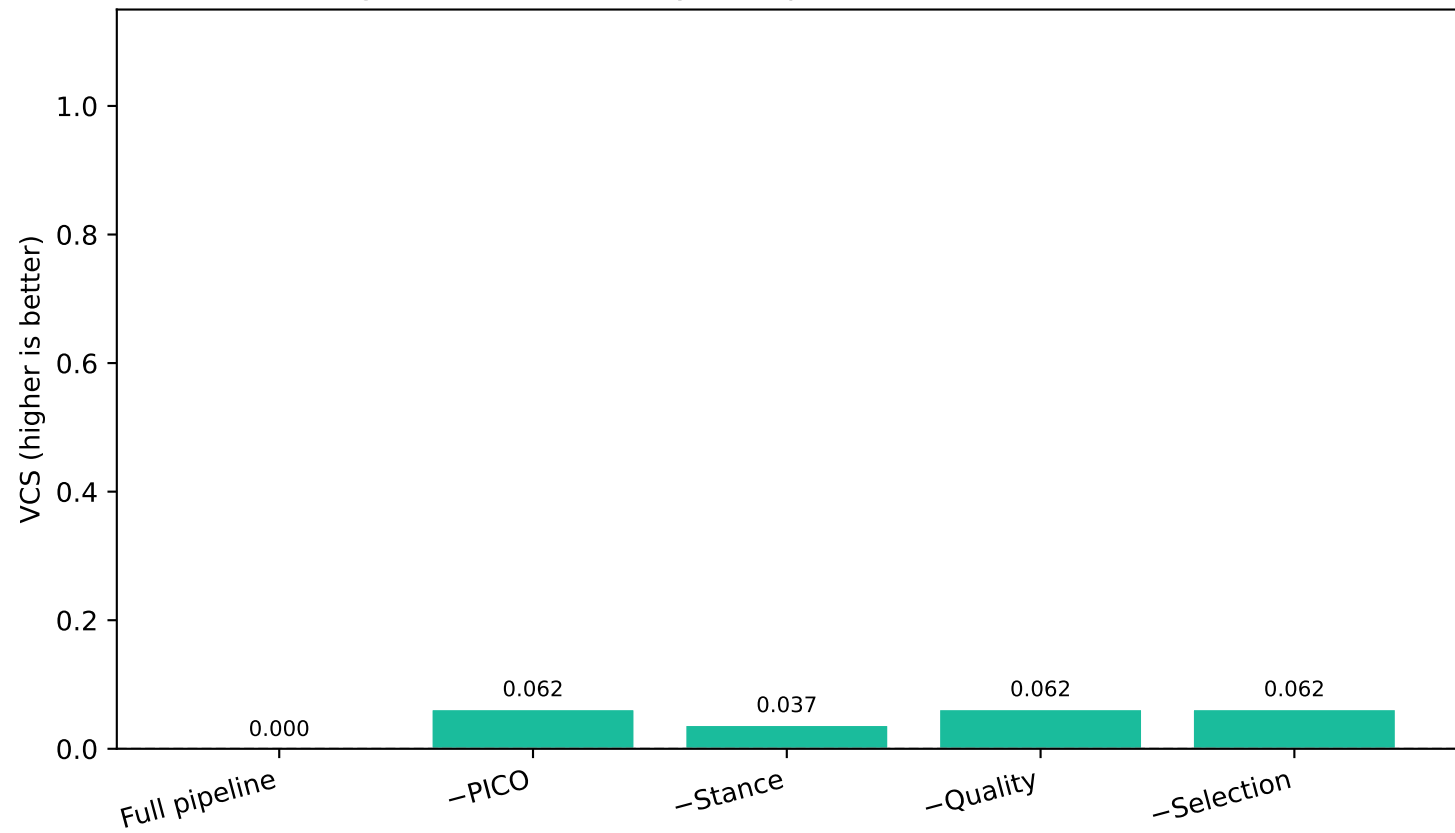
Fig 3 — Ablation Study: Component Contributions to VCS
