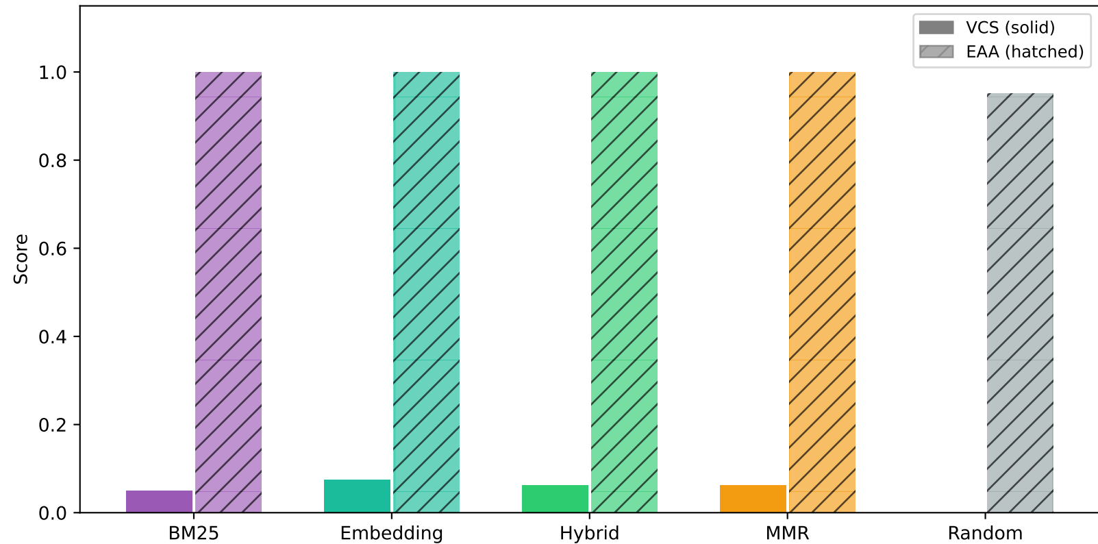
Fig 5 — Retrieval Strategy Comparison
