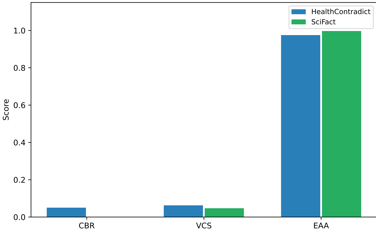
Fig 6 — Cross-Dataset Generalisation (Strategy C)
