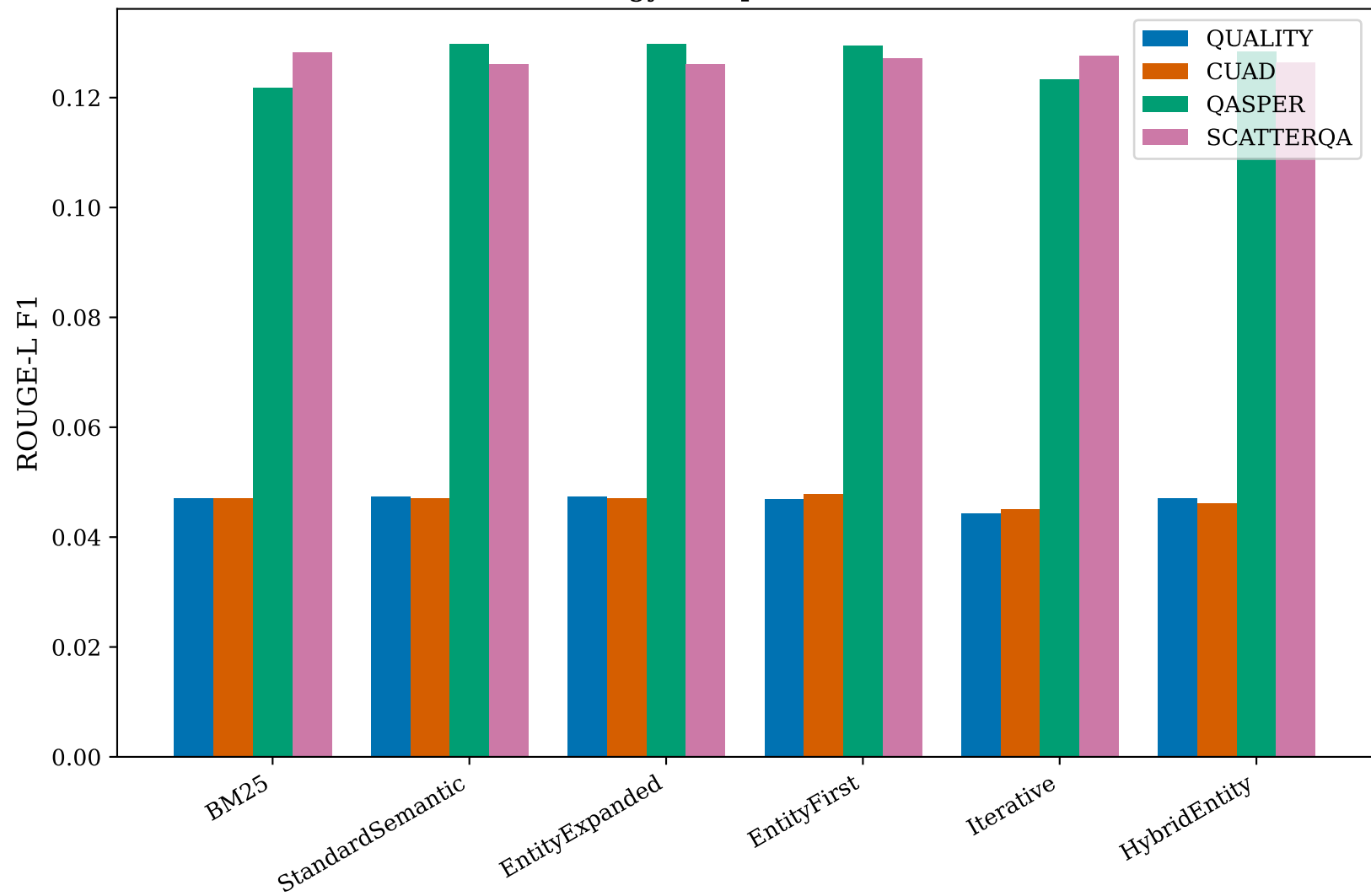
Retrieval Strategy Comparison Across Datasets
