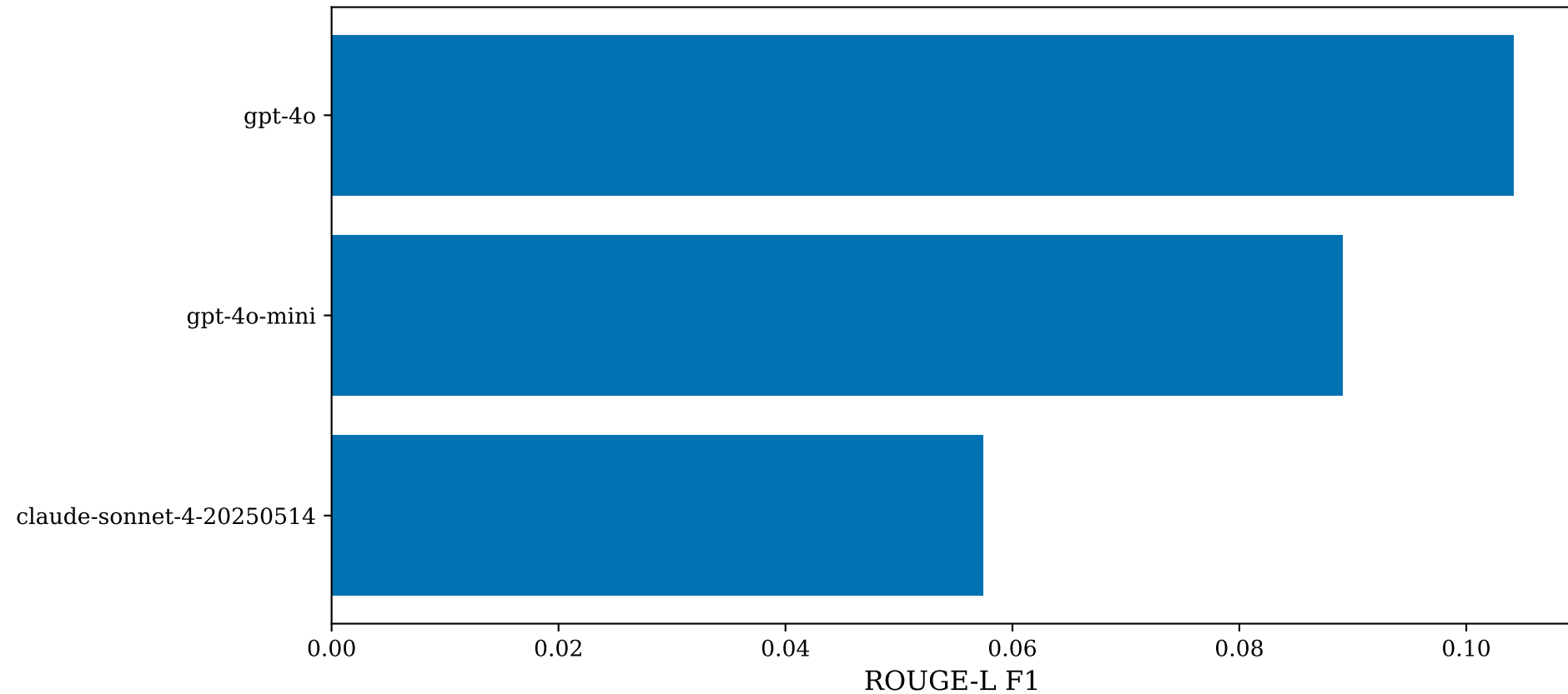
LLM Backbone Comparison (Same Retrieved Chunks)
