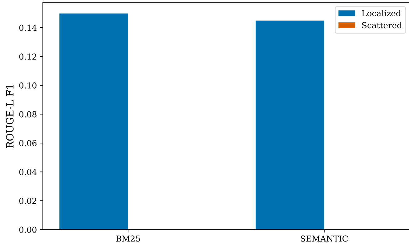
RAG Performance: Localized vs. Scattered Queries
