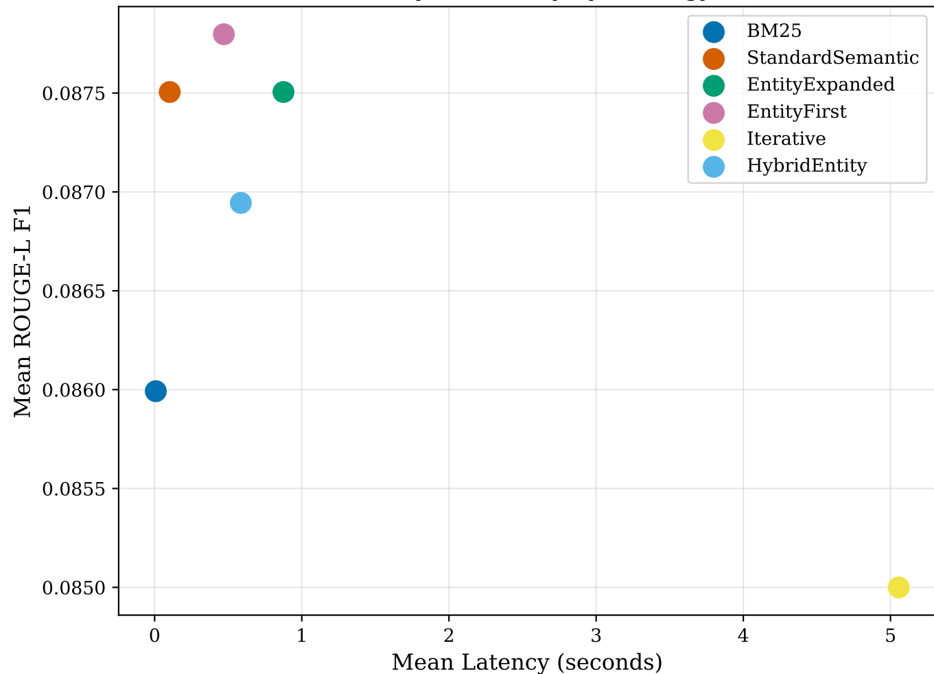
Quality vs Latency by Strategy
