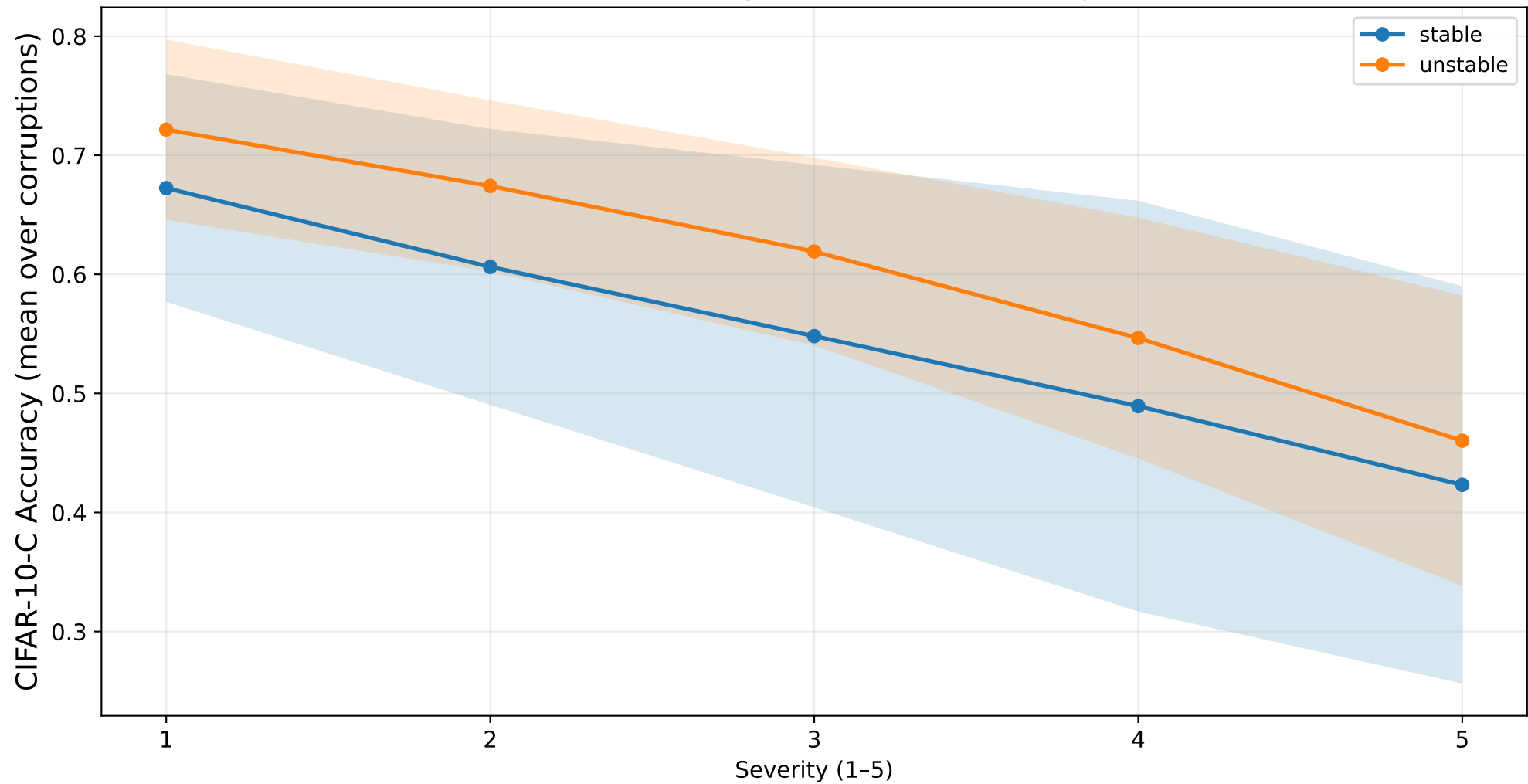
ResNet-18: Corruption robustness vs Severity
