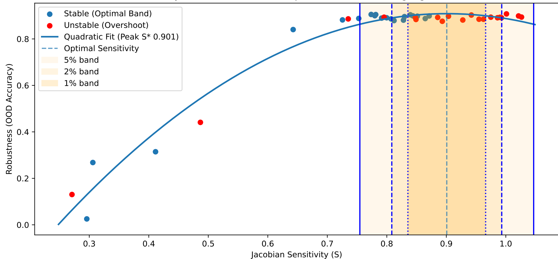
Sensitivity-Robustness Relationship in a Transformer Language Model
