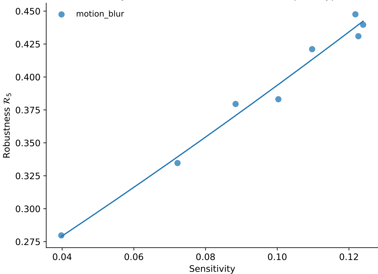
Sensitivity-robustness structure across corruption types
