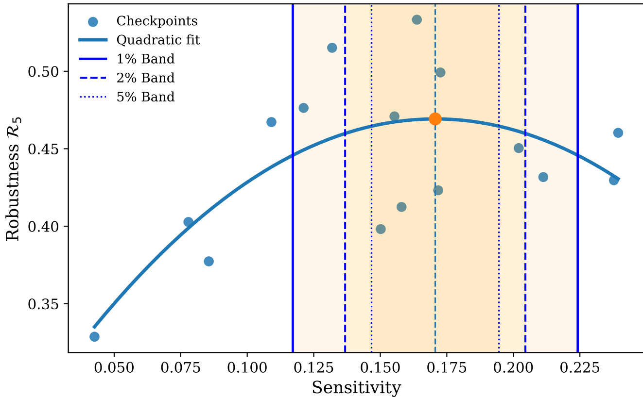
ResNet-18: optimal sensitivity band across \eta
