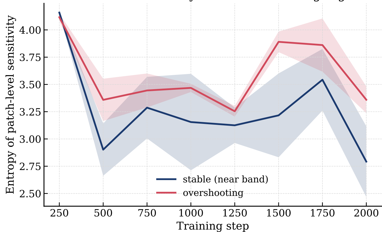
Diffusion of sensitivity in the overshooting regime
