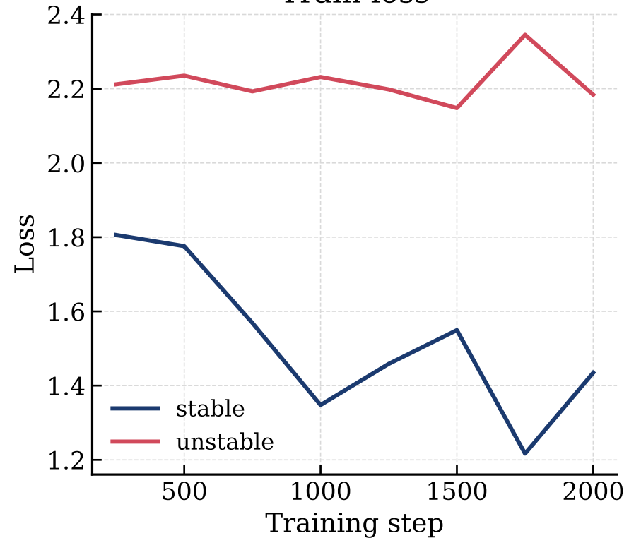
Train loss
