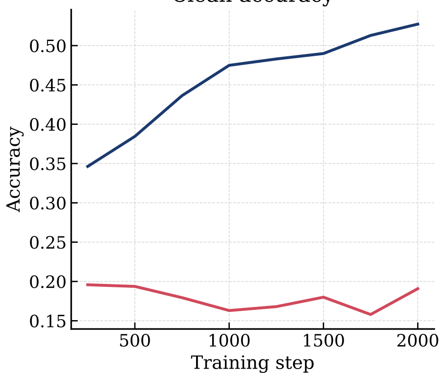
Clean accuracy
