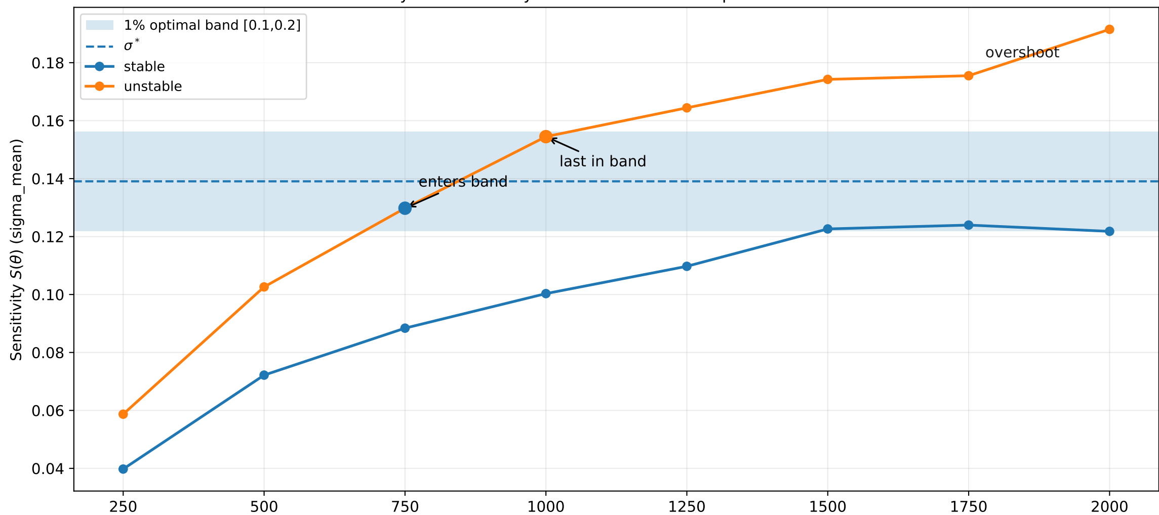
Tiny ViT: Sensitivity band and severe-corruption robustness
