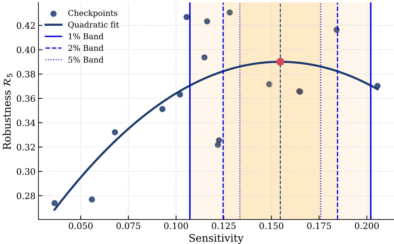
Tiny ViT: optimal sensitivity band across \eta
