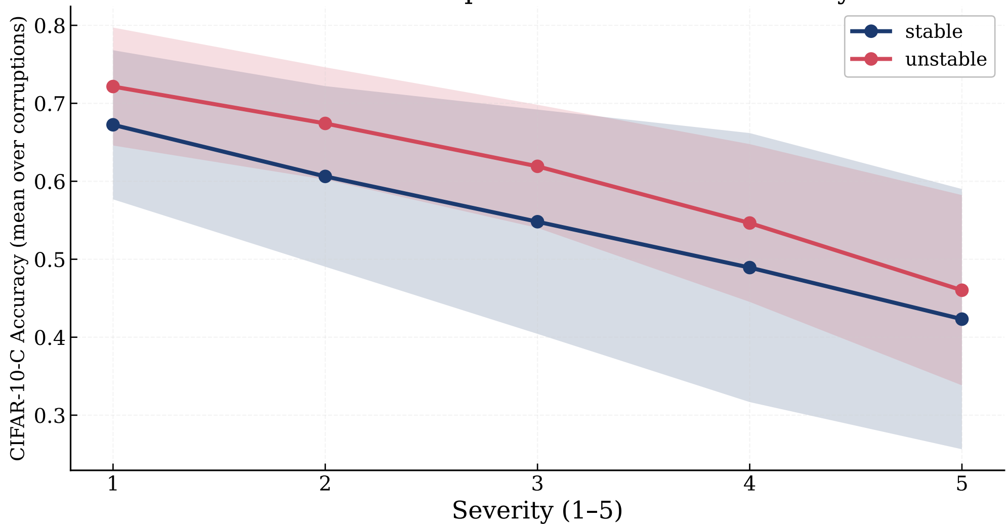
ResNet-18: Corruption robustness vs Severity
