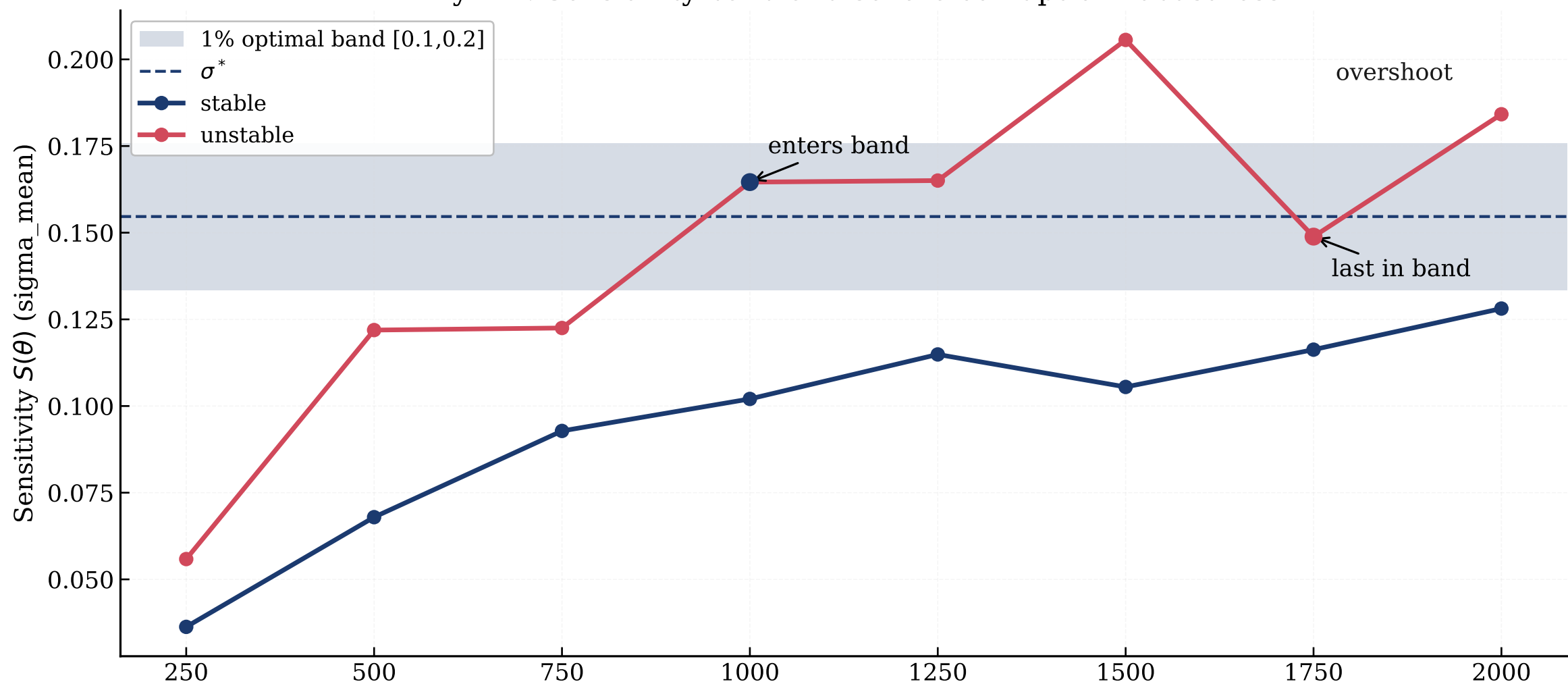
Tiny ViT: Sensitivity band and severe-corruption robustness
