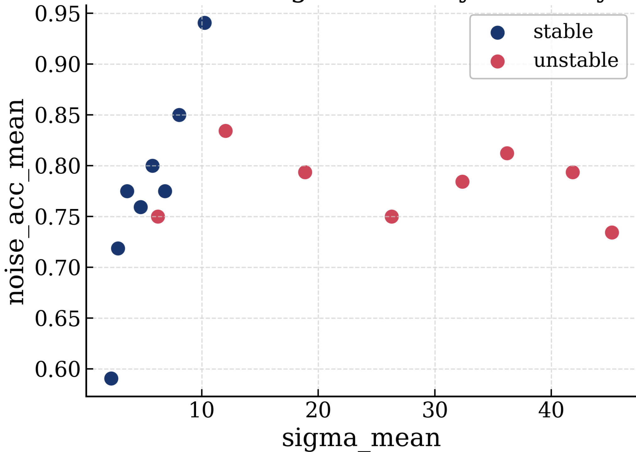
CIFAR-10: sigma vs noisy accuracy
