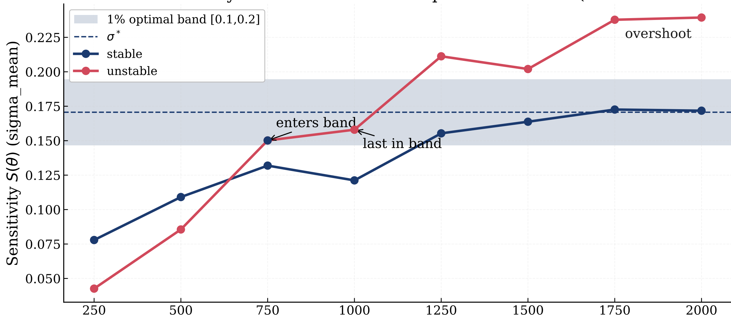
ResNet-18: Sensitivity band and severe-corruption robustness (CIFAR-10-C sev=5)
