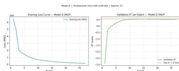
Figure 12: Training loss and validation R^2 per epoch for Model D. The model converged in 27 epochs before early stopping halted training.
