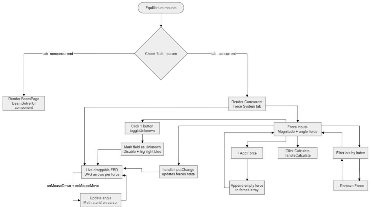
Figure 3.6: Equilibrium of Concurrent Force System Flowchart
