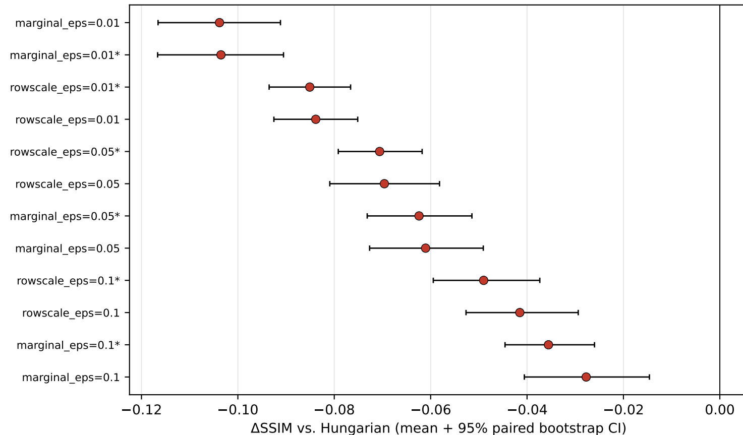
Phase 2 — every Sinkhorn variant loses to Hungarian
