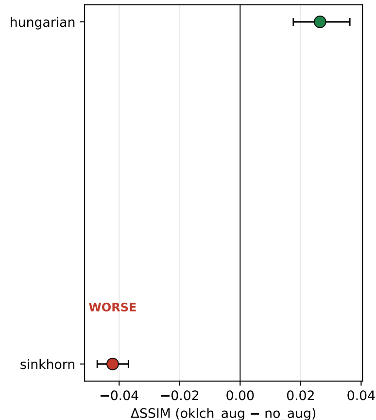
Phase 3 — oklch-aug splits the matchers (N=8×4)
