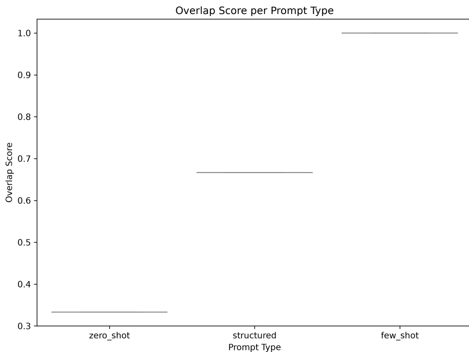
Figure 4.1: Overlap score distribution per prompt type.
