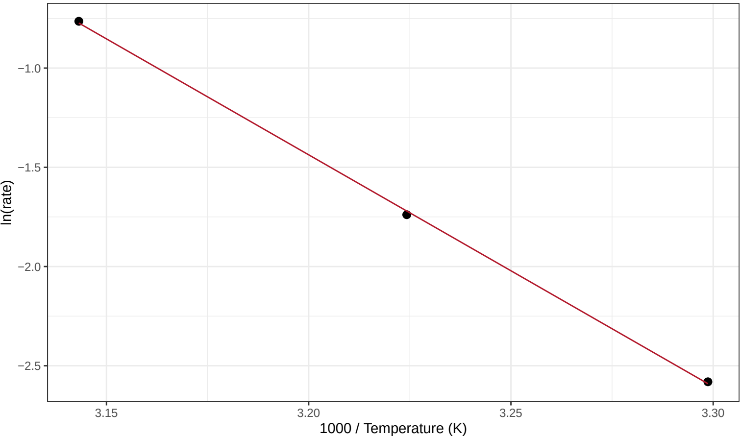
Arrhenius regression
