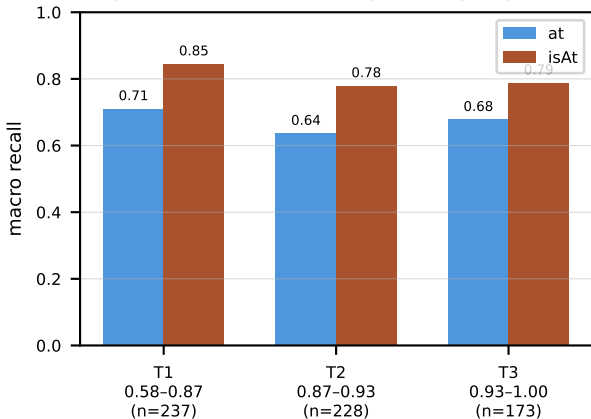
Top-5 ensemble macro-recall per OCR-quality tertile
