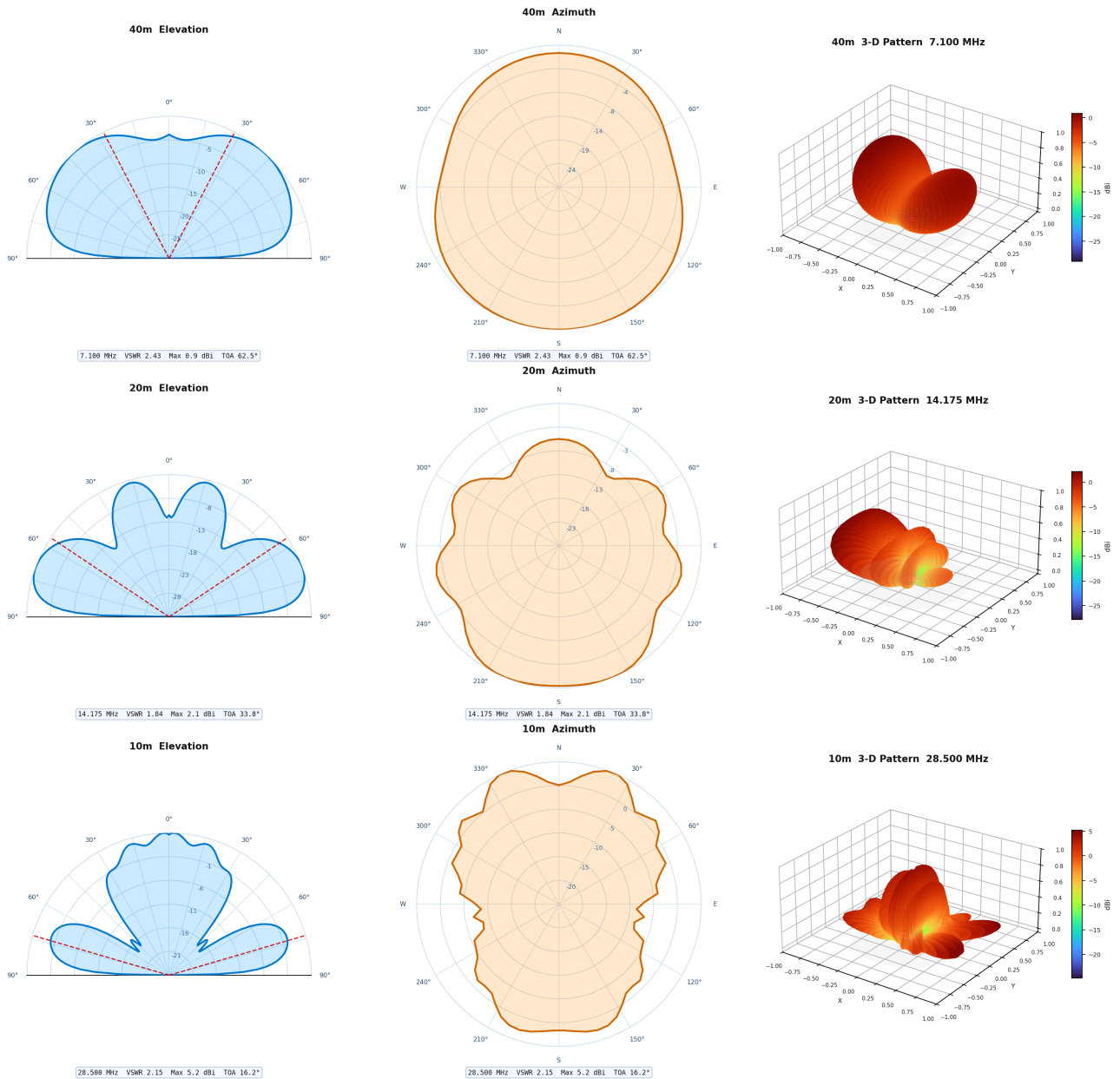
Radiation Diagrams — Wire 38.25 m / CP 9.50 m (45.0°)
