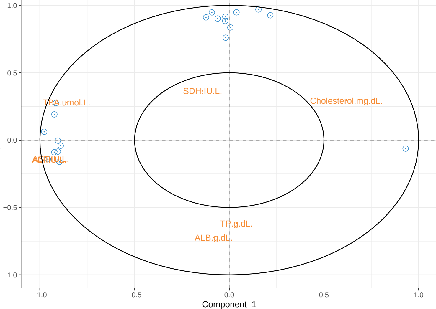
Correlation Circle Plot
