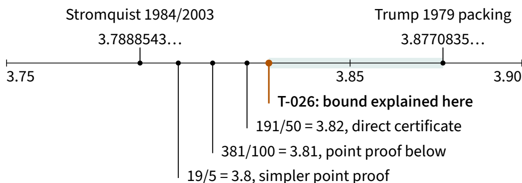
Figure 3. Bounds on s(11) . The shaded band is the gap left by the certificates explained here. At T-026's bound the gap is 0.0506361\dots wide, down from 0.0882292\dots at Stromquist's bound.
