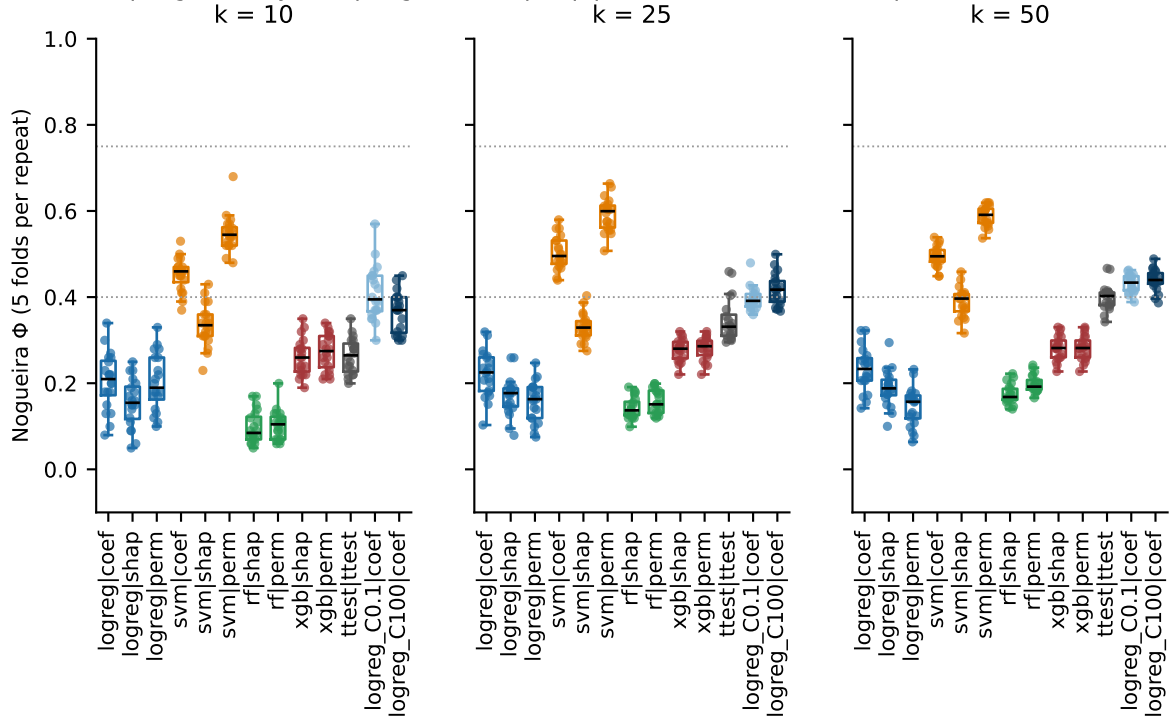
Figure 4. Resampling stability of top-k gene sets per pipeline (dotted: \Phi = 0.40 poor / 0.75 excellent, Nogueira et al. 2018)
