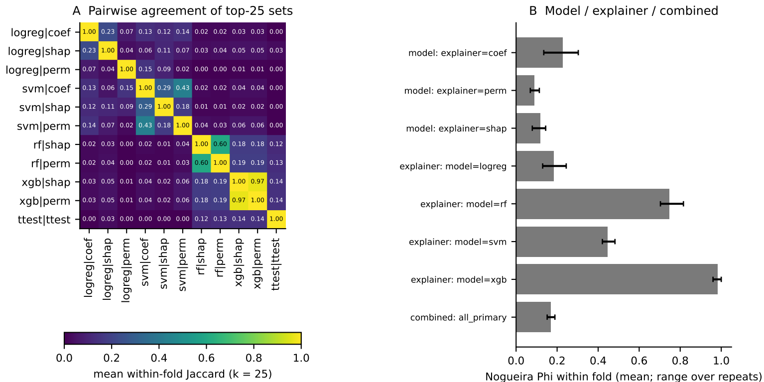
Figure 5. Agreement between analytic choices at the same training data (k = 25)
