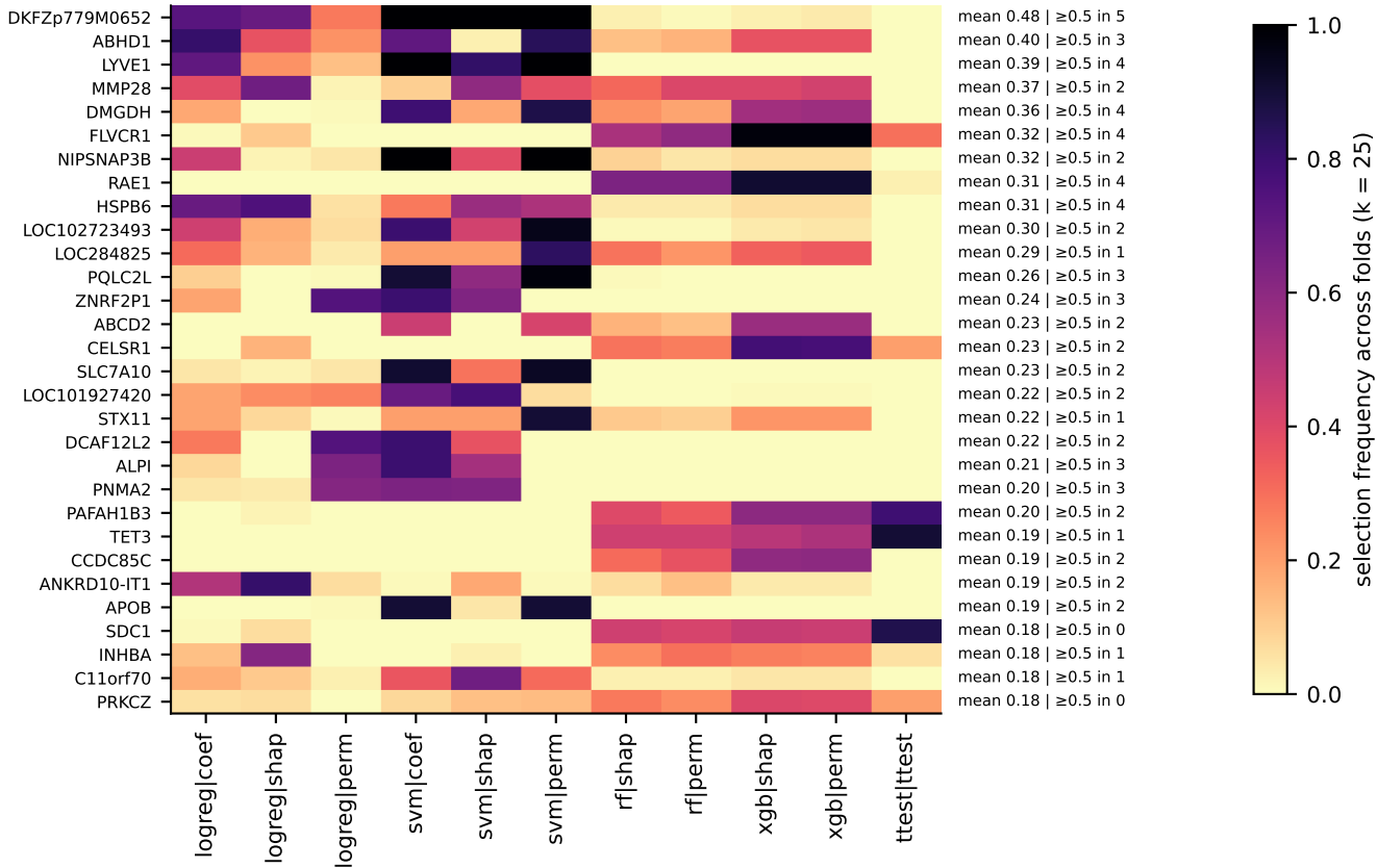
Figure 7. Thirty highest mean-selection-frequency genes (rows) by pipeline (columns); model-supported signals, not biomarkers
