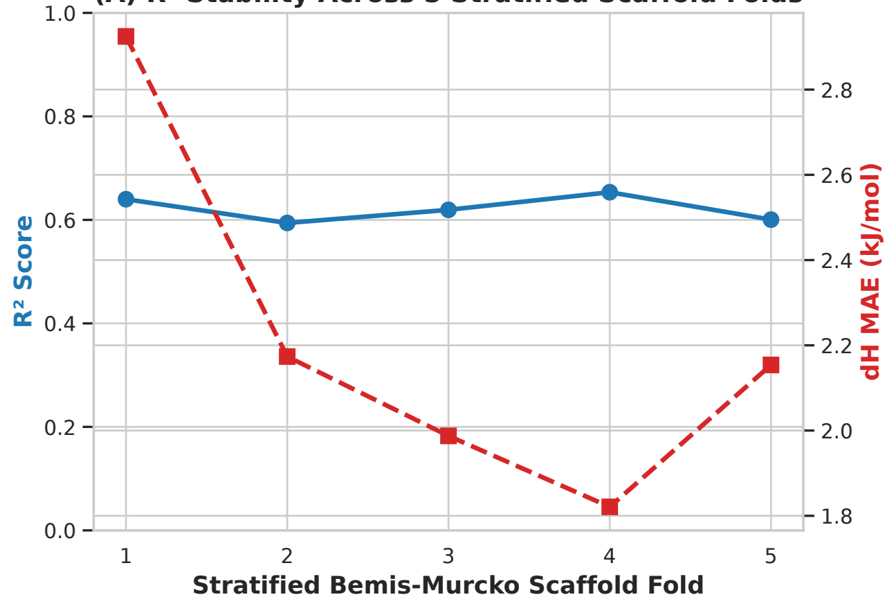
(A) R^2 Stability Across 5 Stratified Scaffold Folds
