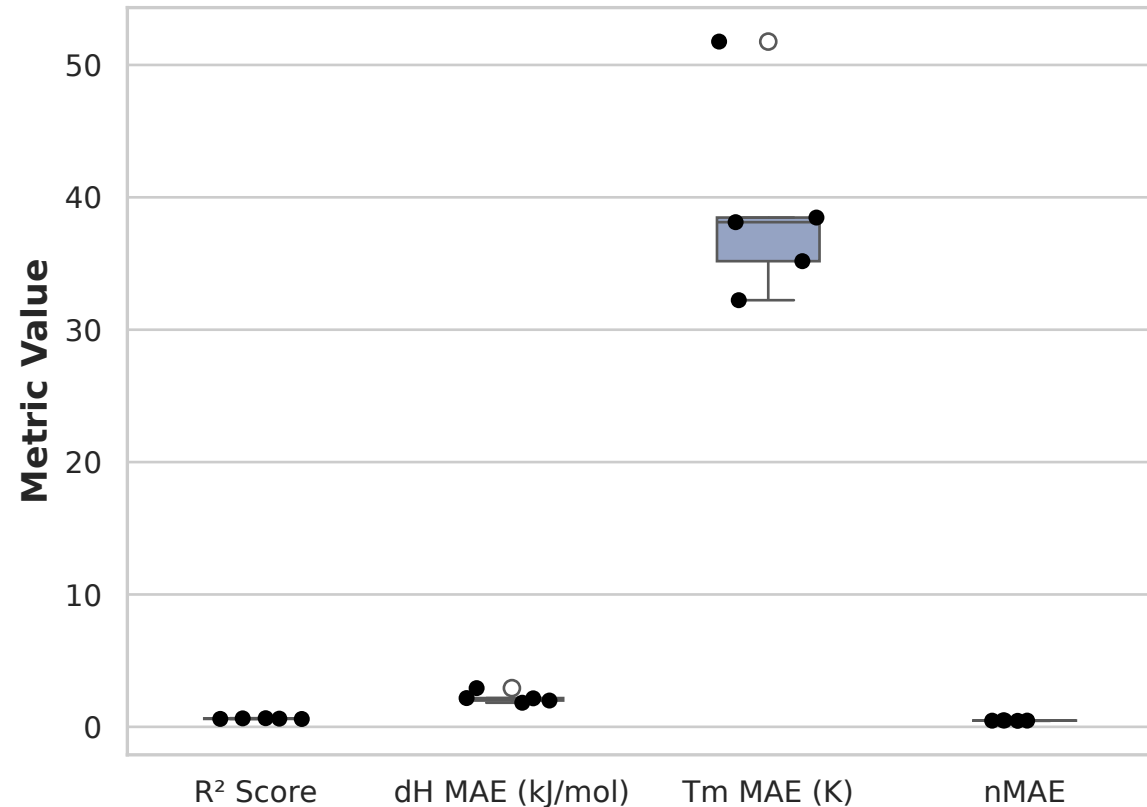
(B) Metric Variance Under Structural Shift
