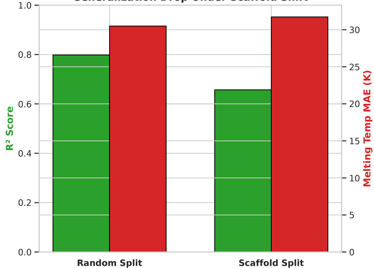
Generalization Drop Under Scaffold Shift
