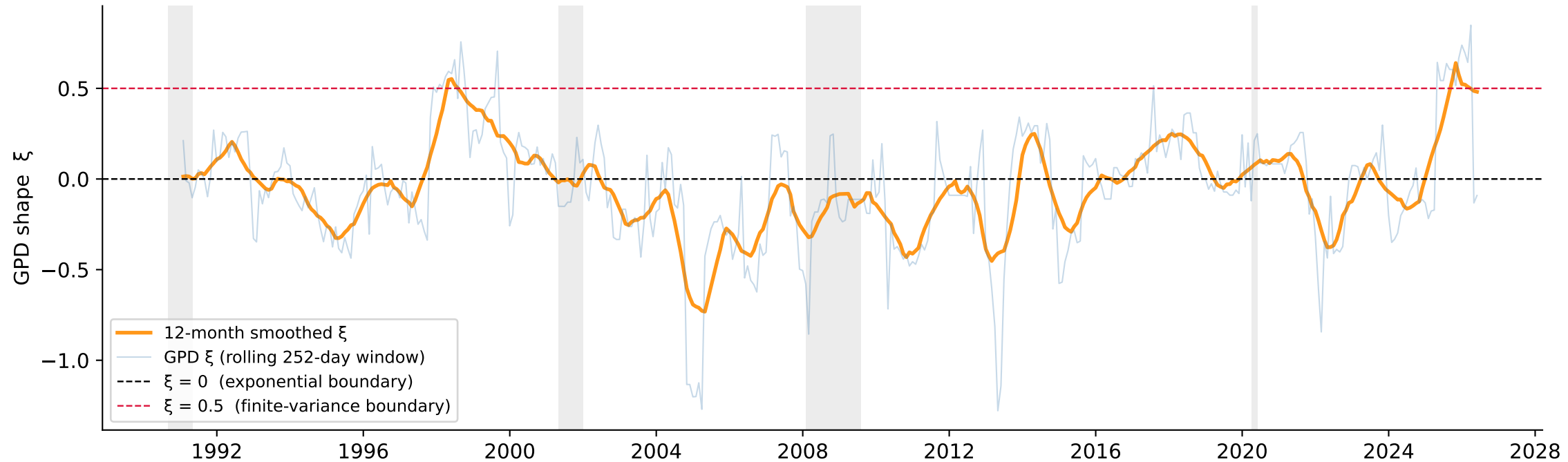
Rolling GPD tail-shape parameter — S&P 500, 252-day window
