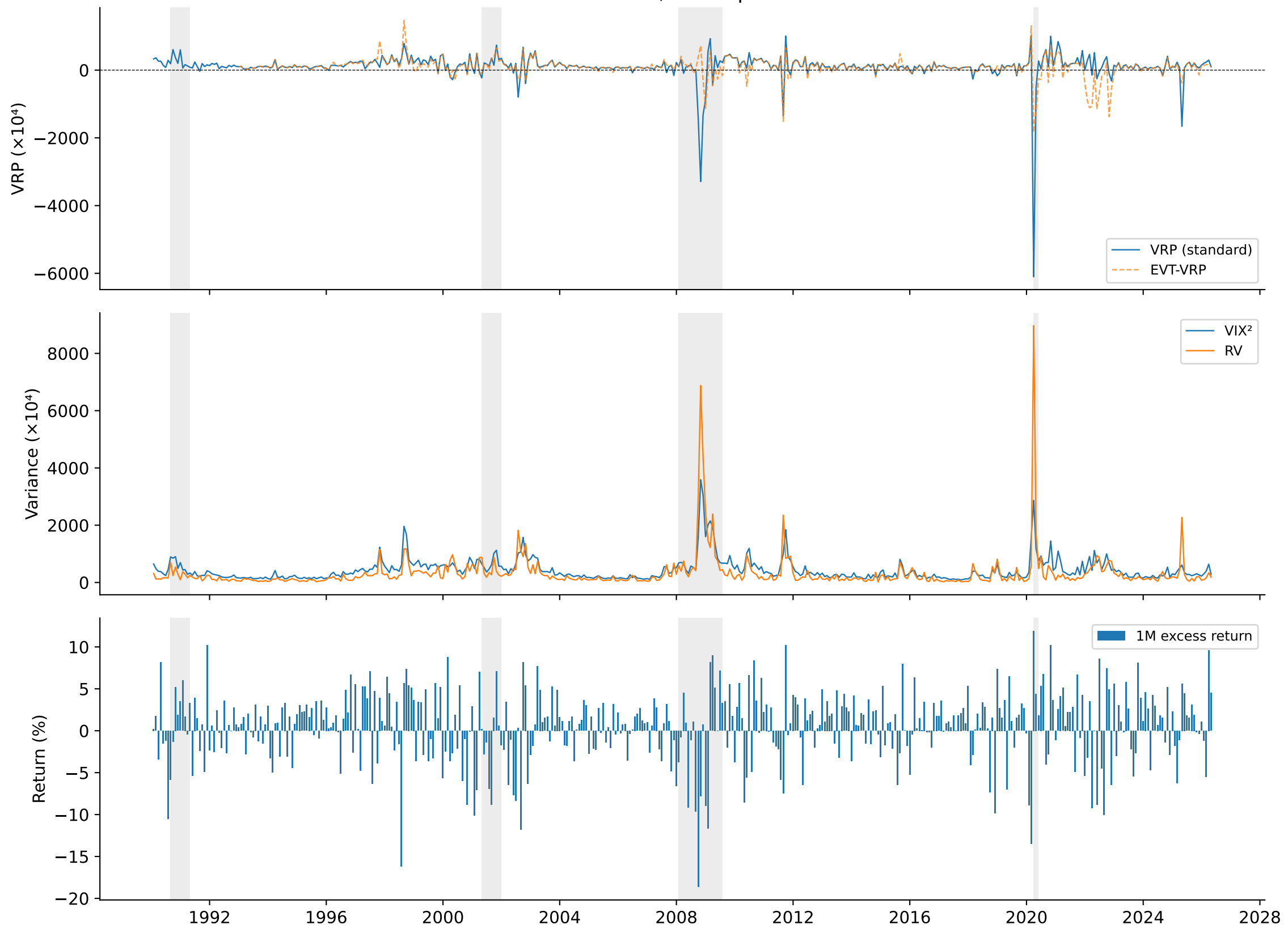
Variance Risk Premium — US, BTZ replication + EVT extension
