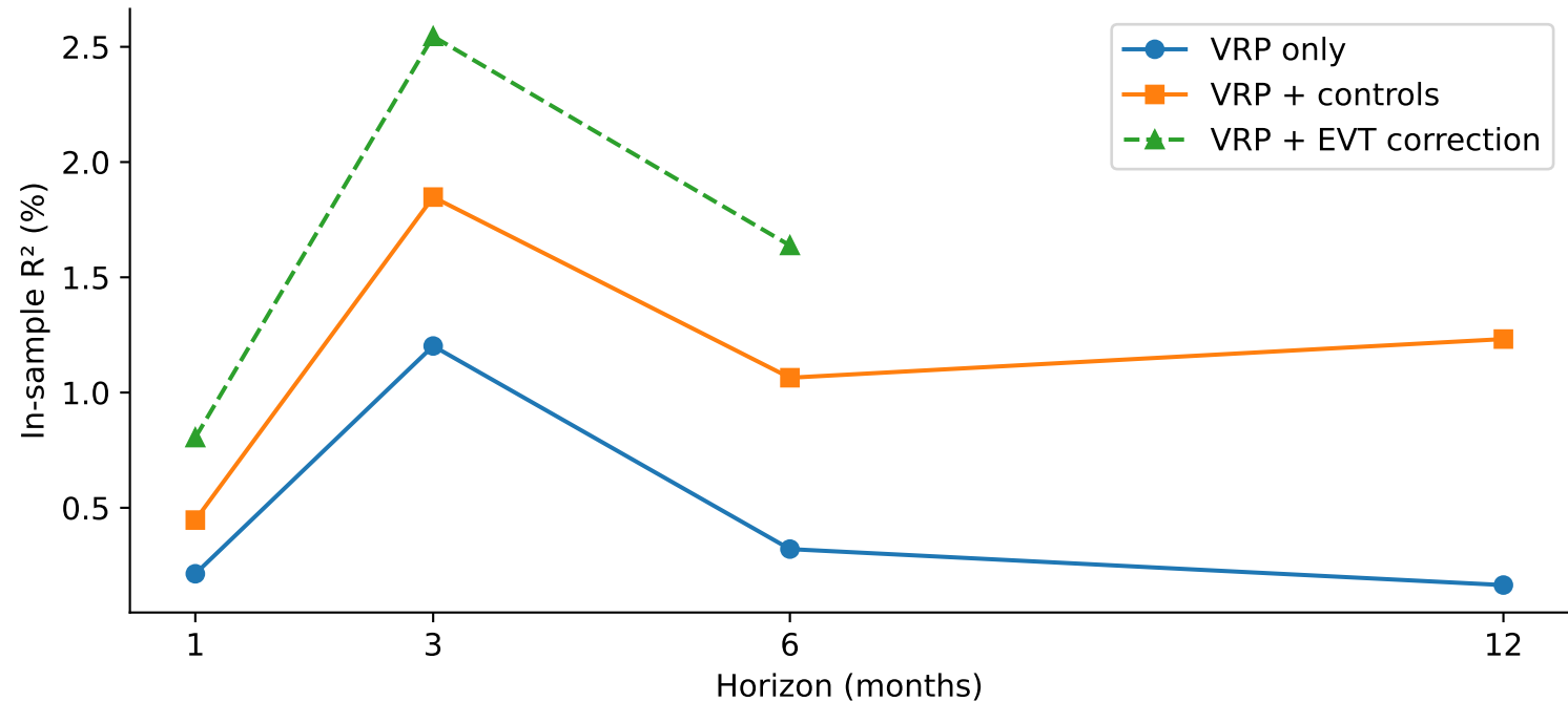
Return predictability of VRP across horizons
