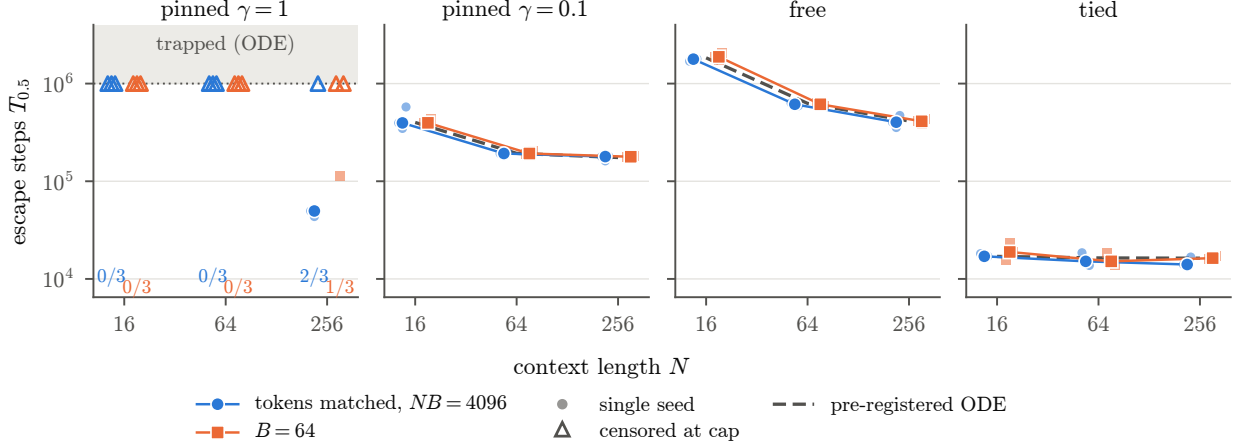
Figure 2: Escape steps T_{0.5} (first step with |m| \geq 0.5 ) against context length N for the four readout protocols ( d = 64 , \eta = 1/d^2 , m_0 = d^{-1/2} ; shared log-log axes). Light markers are single seeds (three per cell), solid markers and lines the median over seeds, for tokens per step fixed ( NB = 4096 , circles) and prompts per step fixed ( B = 64 , squares). Open triangles are runs that had not escaped at the step cap ( 10^6 ) and are drawn at the cap; the counts under the pinned- \gamma = 1 panel are runs escaped out of 3. Dashed lines are the population-ODE escape times (flow time \times d^2 ), fixed before the run ; pinned \gamma = 1 has no finite ODE escape time (trapped, shaded beyond the cap). The free-readout N = 16 cells use the reruns to 2.5 \cdot 10^6 steps (the pre-registered cap was exceeded by the predicted 1.84M steps). At N = 64 both schemes have B = 64 and are the same three runs.
