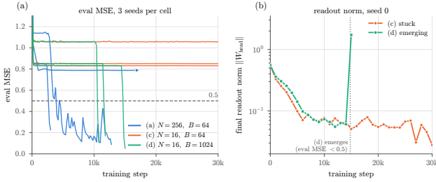
Figure 5. Two-layer softmax transformer, d = 256 , MLP width 32, k^* = 2 . (a) Evaluation MSE for N=256, B=64 ; N=16, B=64 ; and N=16, B=1024 (same tokens per step as the first), three seeds each; one N=256 seed was censored at 17k steps on the plateau. (b) Norm of the final readout for one stuck run ( N=16, B=64 ) and one emerging run ( N=16, B=1024 , same seed): the norm collapses while the skill is unlearned; the regrowth at emergence is a single logged point (norms logged every 1000 steps).
