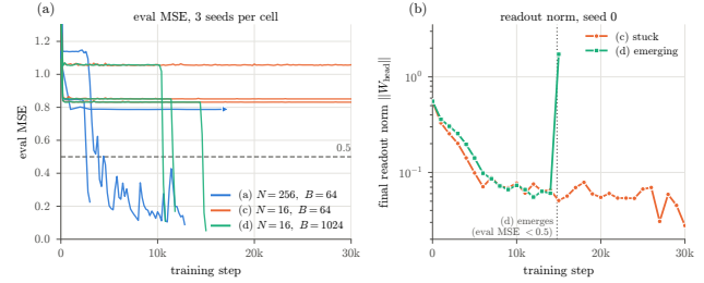
Figure 5. Two-layer softmax transformer, d = 256 , MLP width 32, k^* = 2 . (a) Evaluation MSE for N = 256, B = 64 ; N = 16, B = 64 ; and N = 16, B = 1024 (same tokens per step as the first), three seeds each; one N = 256 seed was censored at 17k steps on the plateau. (b) Norm of the final readout for one stuck run ( N = 16, B = 64 ) and one emerging run ( N = 16, B = 1024 , same seed): the norm collapses while the skill is unlearned; the regrowth at emergence is a single logged point (norms logged every 1000 steps).
