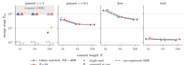
Figure 2. Escape steps T_{0.5} (first step with |m| \geq 0.5 ) against context length N for the four readout protocols ( d = 64 , \eta = 1/d^2 , m_0 = d^{-1/2} ; shared log-log axes). Light markers are single seeds (three per cell), solid markers and lines the median over seeds, for tokens per step fixed ( NB = 4096 , circles) and prompts per step fixed ( B = 64 , squares). Open triangles are runs that had not escaped at the step cap ( 10^6 ) and are drawn at the cap; the counts under the pinned- \gamma = 1 panel are runs escaped out of 3. Dashed lines are the population-ODE escape times (flow time \times d^2 ), fixed before the run; pinned \gamma = 1 has no finite ODE escape time (trapped, shaded beyond the cap). The free-readout N = 16 cells use the reruns to 2.5 \cdot 10^6 steps (the pre-registered cap was exceeded by the predicted 1.82M steps). At N = 64 both schemes have B = 64 and are the same three runs.
