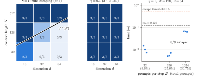
Figure 3. Left: fraction of runs escaping m_0 = d^{-1/2} within 3 \cdot 10^5 steps (fixed readout, 3 seeds per cell; curve: d^*(N) of Prop. 2; for \gamma = 0.1 the curve lies above the grid). Right: at \gamma = 1 , N = 128 , d = 64 no run escapes for B \in \{32, 256, 1024\} prompts per step (total prompts \times 1 , \times 2.7 , \times 3.2 ) and the final overlap falls below m_0 : more prompts do not substitute for context length.
