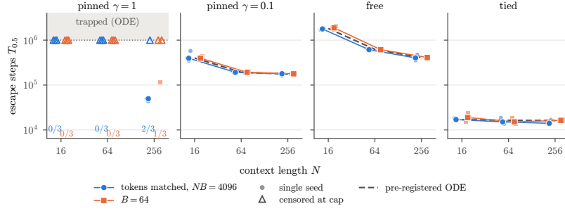
Figure 1. Escape steps T_{0.5} against context length N for the four readout protocols ( d = 64 , \eta = 1/d^2 , m_0 = d^{-1/2} ). Light markers are single seeds (three per cell), solid markers and lines the median over seeds, for tokens per step fixed ( NB = 4096 , circles) and prompts per step fixed ( B = 64 , squares). Open triangles are runs that had not escaped at the step cap ( 10^6 ) and are drawn at the cap; the counts under the pinned- \gamma = 1 panel are runs escaped out of 3. Dashed lines are the population-ODE escape times (flow time \times d^2 ), fixed before the run.
