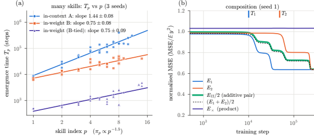
Figure 4. (a) Emergence time (drop midpoint) of skill p versus skill index for the in-context model (slope 1.44 \pm 0.08 ), the capacity-matched in-weight baseline (slope 0.75 \pm 0.08 ) and the 2-homogeneous in-weight student (slope 0.75 \pm 0.09 ), \pi_p \propto p^{-1.5} , three seeds each; unlearned skills omitted. (b) Composition (Exp. 3, one seed): normalised MSE on skill-1 prompts, skill-2 prompts, the additive pair (halved) and the product pair; the dotted curve is half the sum of the single-skill losses and lies on the pair curve. Plateaus at 0.64 are the fixed-readout floor (1 - \Gamma n)^2 , not zero.
