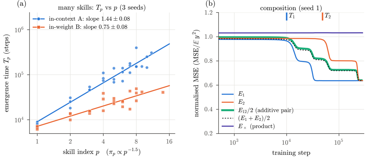
Figure 3: (a) Emergence time (drop midpoint) of skill p versus skill index for the in-context model (slope 1.44 \pm 0.08 ) and the capacity-matched in-weight baseline (slope 0.75 \pm 0.08 ), \pi_p \propto p^{-1.5} , three seeds; unlearned skills omitted. (b) Composition (Exp. 3, one seed): normalised MSE on skill-1 prompts, skill-2 prompts, the additive pair (halved) and the product pair; the dotted curve is half the sum of the single-skill losses and lies on the pair curve. Plateaus at 0.64 are the fixed-readout floor (1 - \Gamma n)^2 , not zero.
