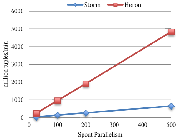
Figure 12: Throughput with acknowledgements disabled
