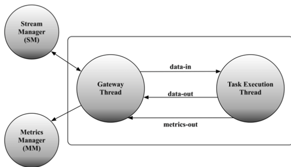
Figure 5: Heron Instance
