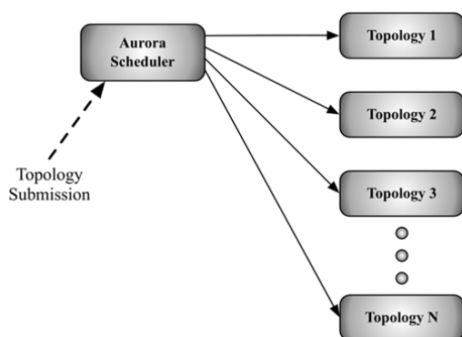
Figure 3: Heron Architecture
