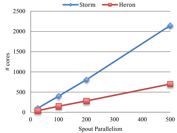
Figure 11: CPU usage with acknowledgements
