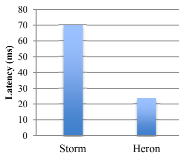
Figure 15: End-to-end latency with acknowledgements
