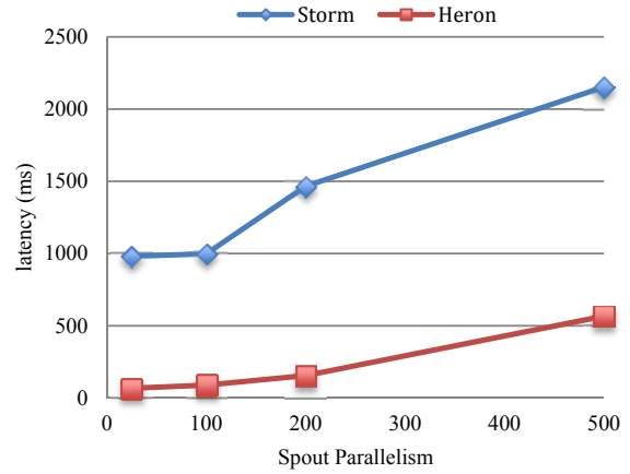
Figure 10: End-to-end latency with acknowledgements
