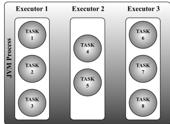
Figure 2: Storm Worker
