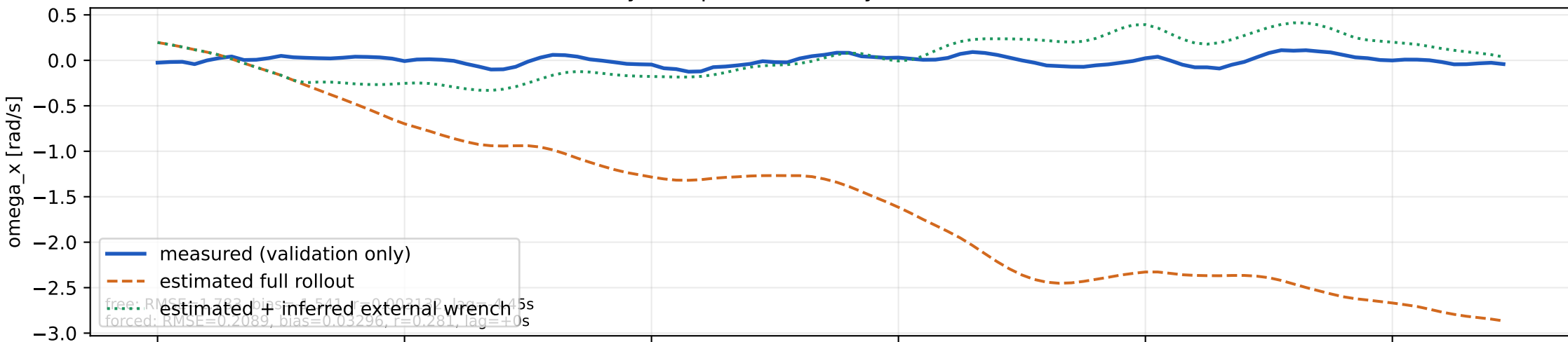
Gyroscope (not used by estimator loss)
