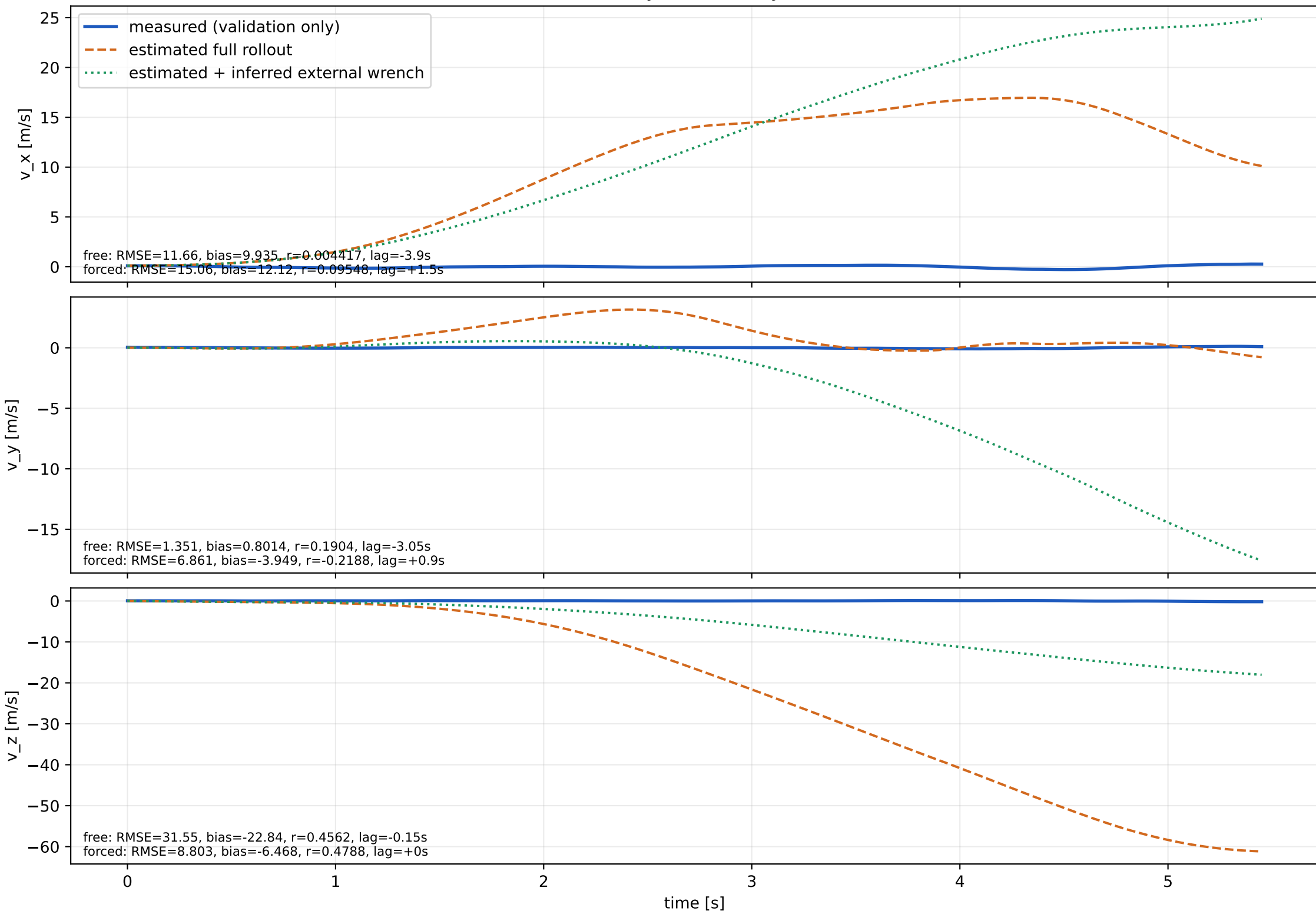
World-frame velocity (not used by estimator loss)
