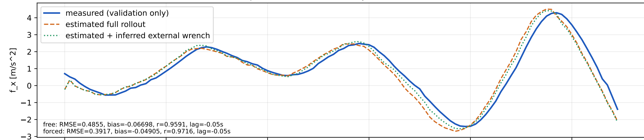
Specific force (not used by estimator loss)
